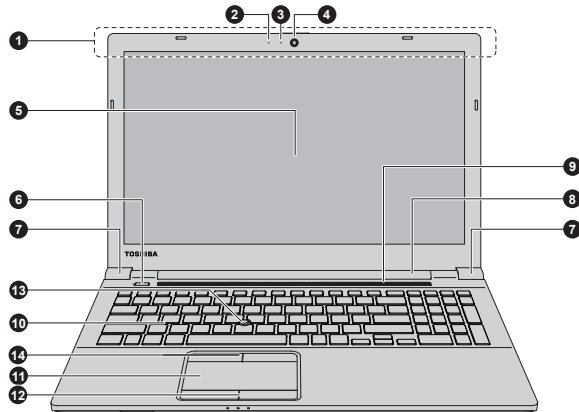
Figure 3-6 The front of the computer with the display panel open
